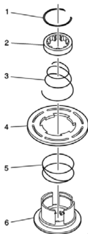
Two/Four Wheel Drive Synchronizer Hub Disassemble
